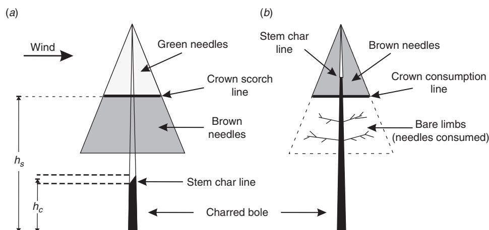
Fig. 6. Variation in direct effects of (a) low- to (b) high-intensity surface fires on tree crowns and stem boles (adapted from Storey and Merkel 1960).
