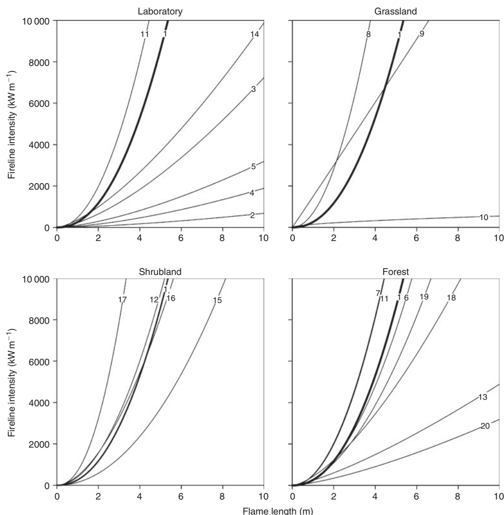
Fig. 4. Graphical representation of Byram's (1959) fireline intensity–flame length relationship (represented by curve 1) and other models reported in the literature. Refer to Table 1 for details of each plotted relationship.
