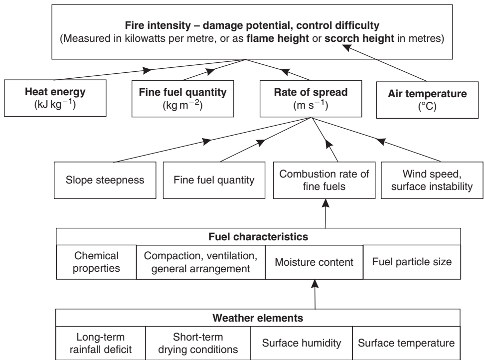
Fig. 2. Schematic diagram illustrating the various elements contributing to fireline intensity and in turn flame height and crown scorch height (after Richmond 1981).
