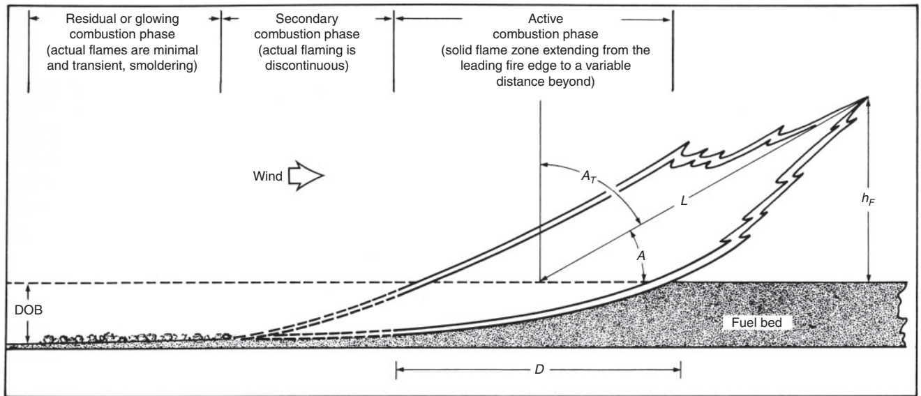
Fig. 3. Cross-section of a stylised, wind-driven surface head fire on level terrain illustrating the energy or heat-release stages during and following passage of the flame front, flame length ( L ), flame height ( h_F ), flame angle ( A ), flame tilt angle ( A_T ), horizontal flame depth ( D ), and the resulting depth of burn (DOB) (from Alexander 1982).
