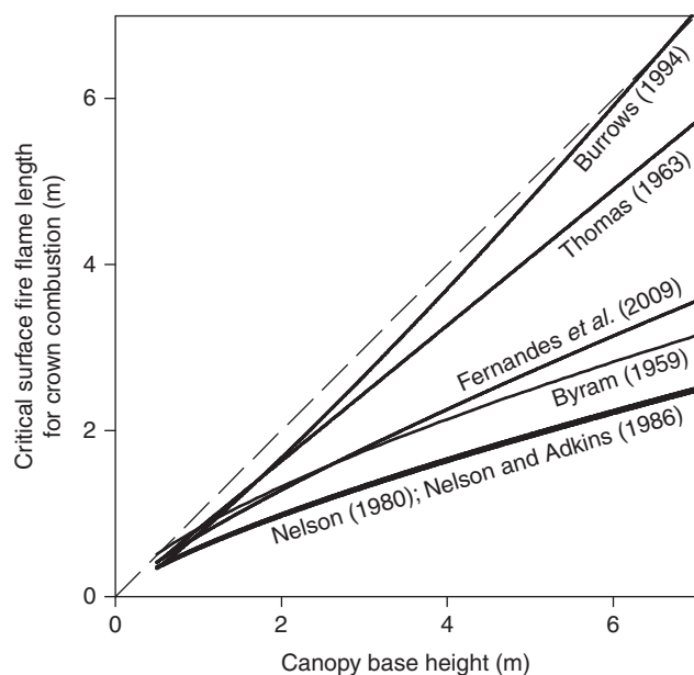
Fig. 5. Critical surface fire flame length for crown combustion in a conifer forest stand as a function of canopy base height according to various flame length–fireline intensity models for forest fuel complexes based on Van Wagner’s (1977) crown fire initiation model. A foliar moisture content of 100% was assumed in all cases. The dashed line represents the boundary of exact agreement between flame length or height and canopy base height.
