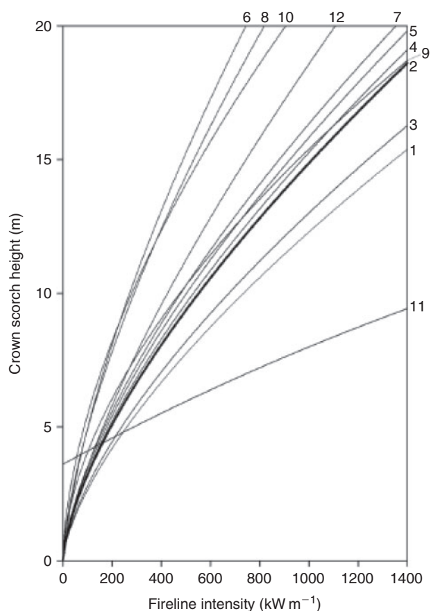
Fig. 10. Graphical representation of Van Wagner's (1973) crown scorch height–fireline intensity relationship (represented by curve 2) and other models reported in the literature. Refer to Table 2 for details of each plotted relationship.
