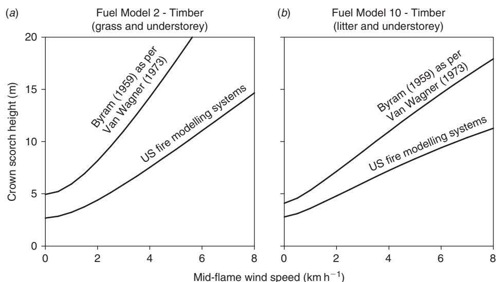
Fig. 7. Crown scorch height as per Van Wagner's (1973) model as a function of mid-flame wind speed for two US fire behaviour fuel models (Anderson 1982) based on different methods of calculating fireline intensity (i.e. Byram 1959 as per Van Wagner 1973 v. US fire modelling systems). The following environmental conditions were held constant: slope steepness, 0%; fine dead fuel moisture, 4%; 10- and 100-h time-lag dead fuel moisture contents, 5 and 6%; live fuel moisture content, 30%; and ambient air temperature, 25°C. The associated 10-m open winds would be a function of forest structure and can be approximated by multiplying the mid-flame wind speed by a factor varying between 2.5 (open stand) and 6.0 (dense stand with high crown ratio) (Albini and Baughman 1979).
