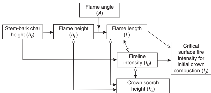
Fig. 1. The inter-relationships involved among commonly used descriptors of surface fire behaviour and fire impacts covered in this review. The solid arrowheads indicate primary relationships established from field data. The hollow arrowheads represent derivations obtained from the primary relationships by solving the equation for the independent variable or using a combination of two primary relationships.
