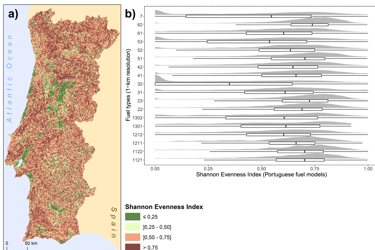
Figure 2: Spatial distribution of a) the Shannon Evenness Index computed using the Portuguese fuel models on the 1-km 2 map of Aragoneses et al. (2023); and b) half-violin plots and boxplots of the same index by fuel types determined by the authors.
