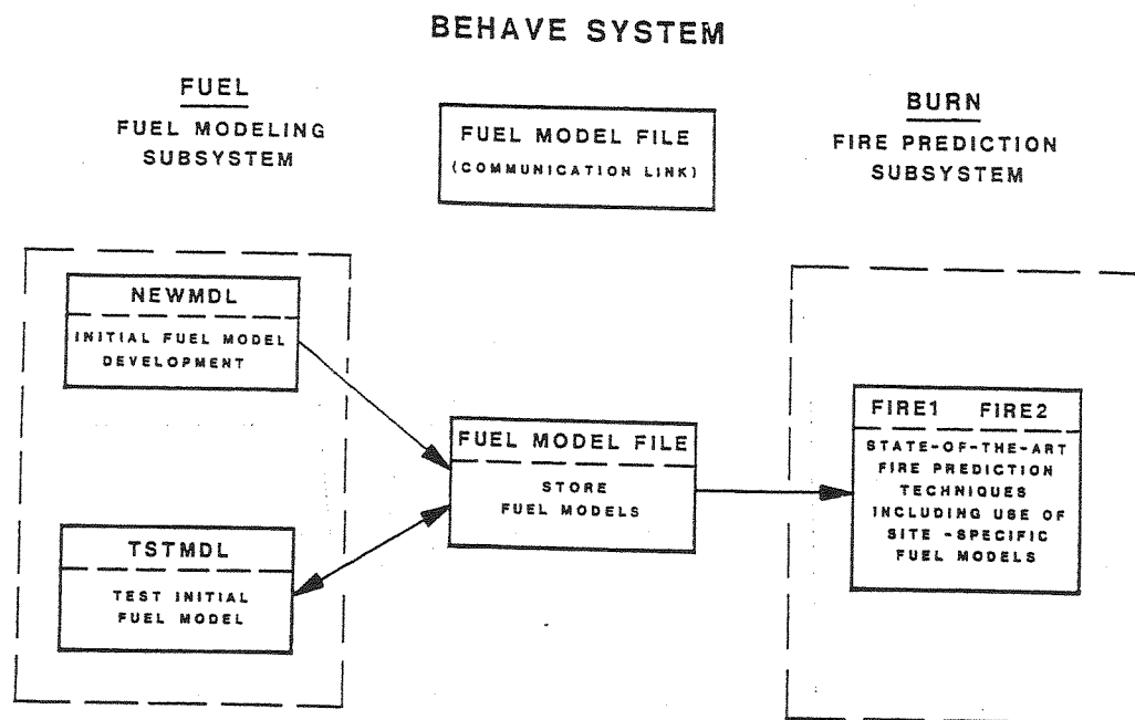
Figure 2.—The fuel model file is the communication link between the two BEHAVE subsystems, FUEL and BURN.
