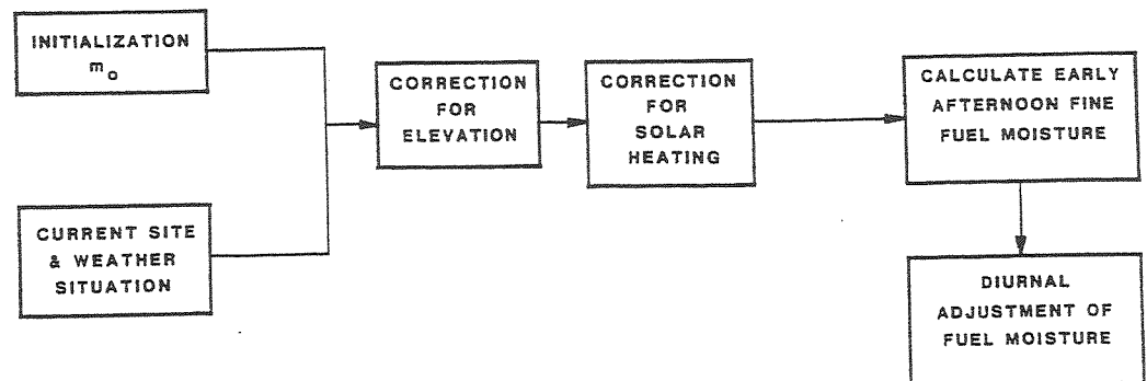
Figure 8.—General flow diagram of the fine fuel moisture model (from Rothermel and others in press).
