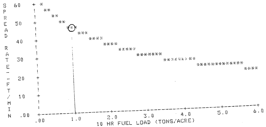
Figure 6.—Graph from TSTMDL showing the effect of a change in 10-h fuel load on spread rate predictions when fuel moisture is held constant.
