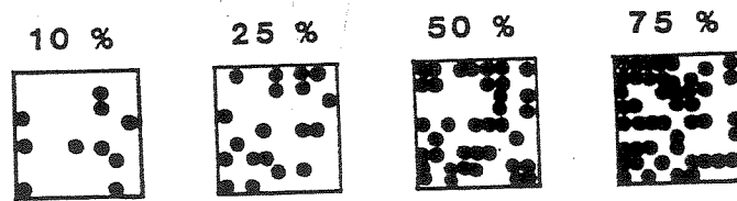
Figure 11.—Aid to estimating canopy closure, an input to SITE.
