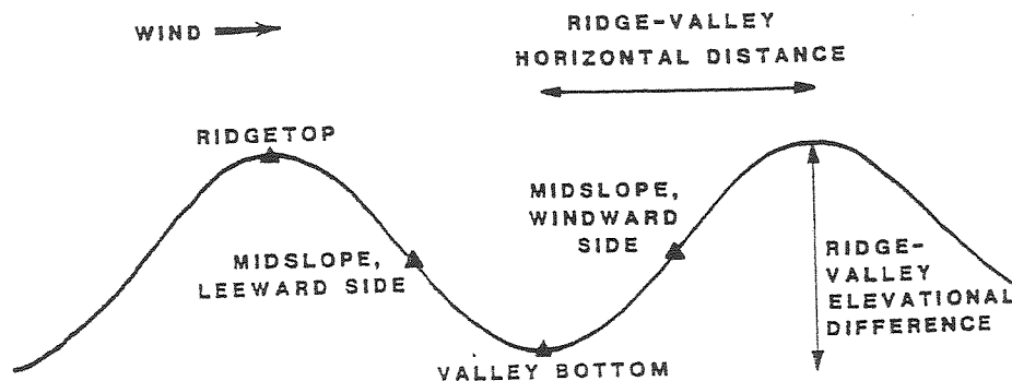
Figure 18.—Mountainous terrain and spotting source location for the maximum spotting distance model.
