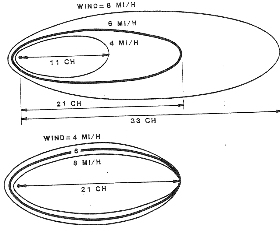
Figure 16.—(A) Fire shapes that correspond to the run in exhibit 18A; (B) fire shapes that correspond to the run in exhibit 18B.
