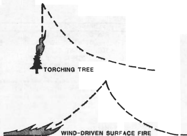
Figure 18 —A firebrand from a torching tree or a burning pile is lifted straight up and then carried by the prevailing wind. This is compared to a firebrand from a wind-driven surface fire, which is carried some distance downwind from the fire-front where the thermal originated before it is carried by the prevailing wind.
