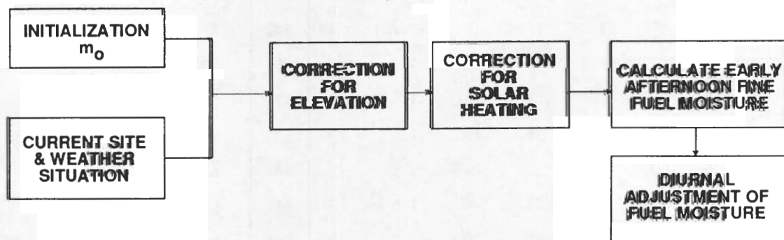
Figure 29—General flow diagram of the fine fuel moisture model that is in SITE and MOISTURE.
